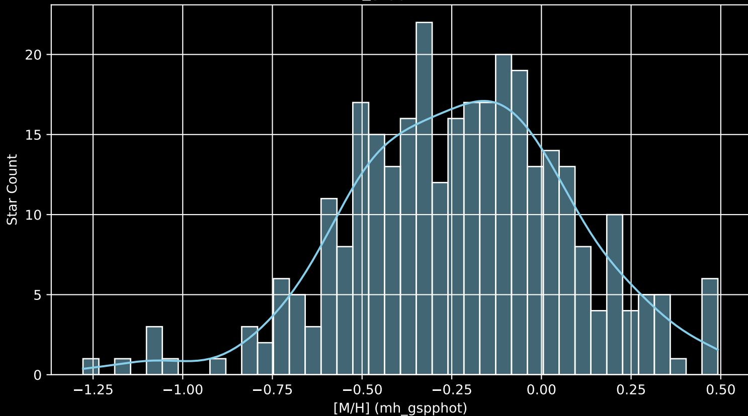
APOGEE DR17 Field: [179-57 [M/H] (mh_gspphot) (n= 312)
