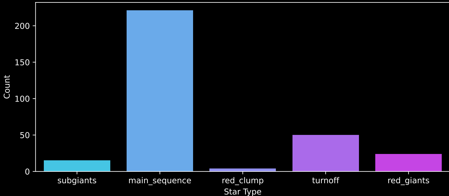
APOGEE DR17 Field: [179-57] Count plot of Star Type
