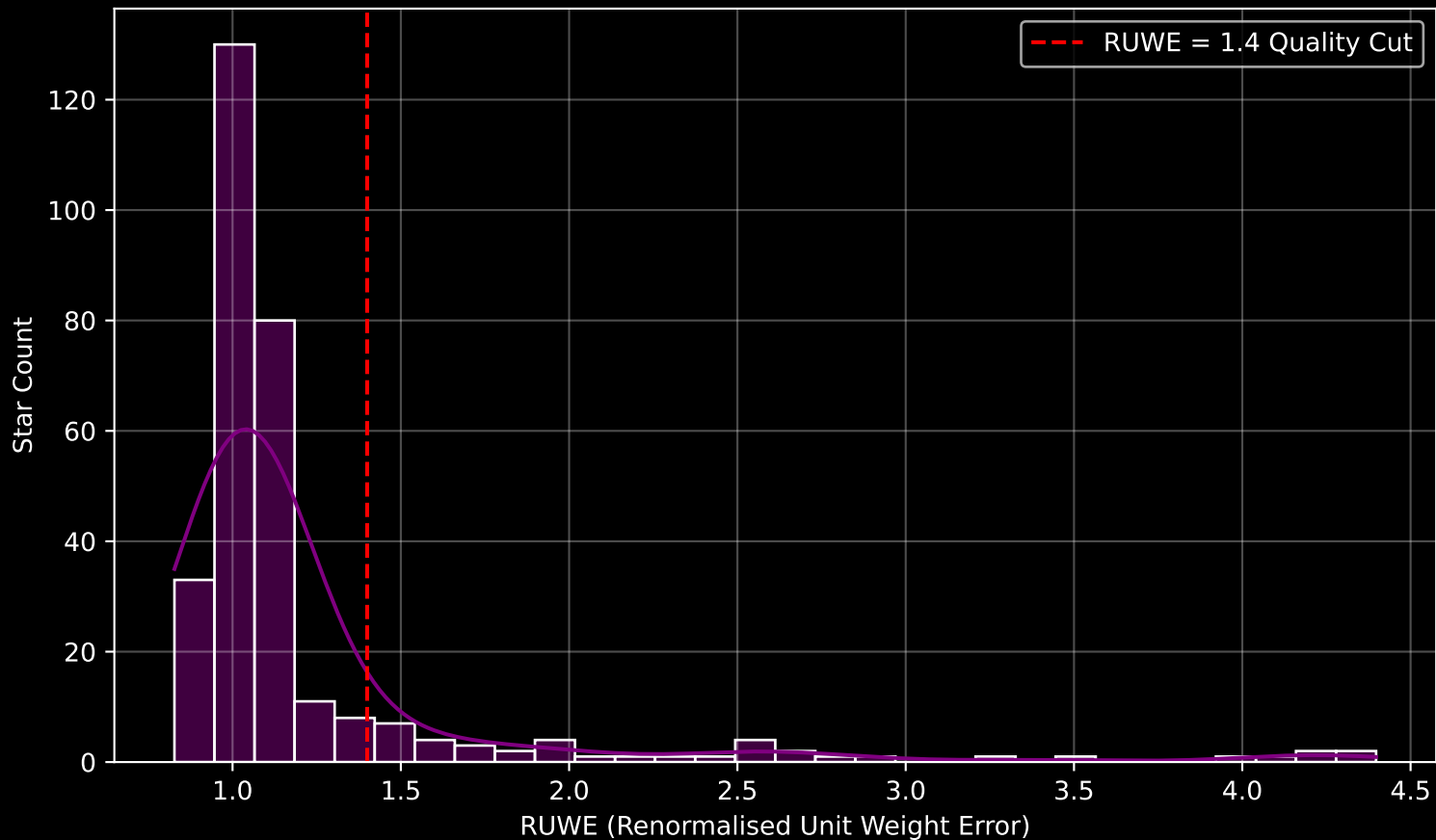
GAPOGEE DR17 Field [179-57] RUWE Distribution (n= 302)
