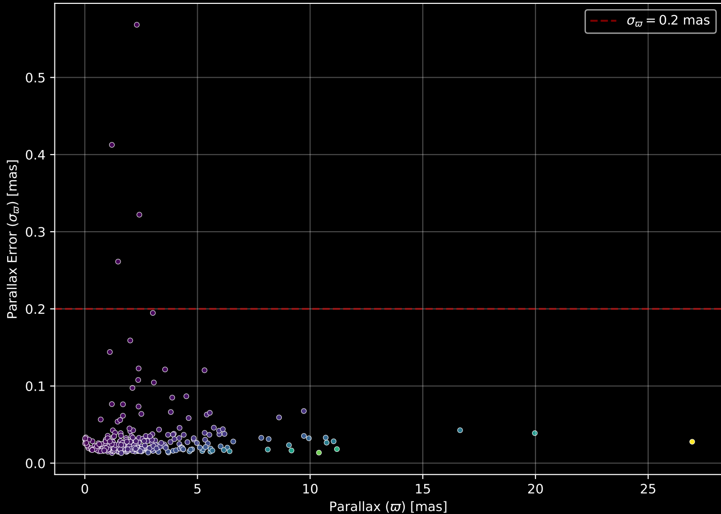
APOGEE DR17 Field: [179-57] Parallax Quality (n= 314)
