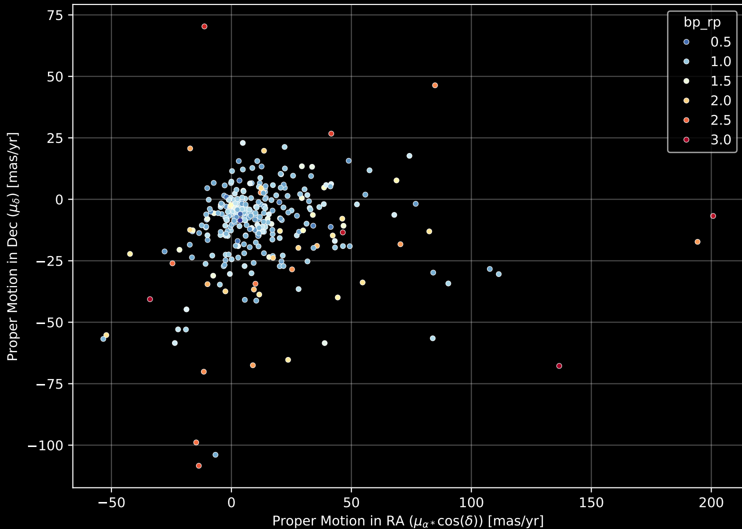
APOGEE DR17 Field: [179-57] Proper Motion Diagram (n= 314)
