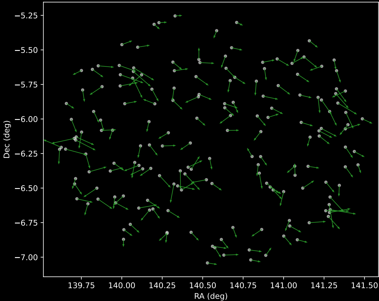
APOGEE DR17 Cluster 4 Proper Motion Vectors (n=174)
