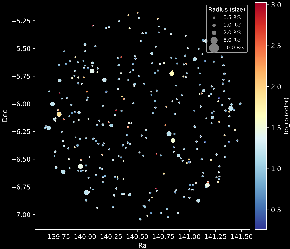
APOGEE DR17 Field: [179-57] Stars: 314
